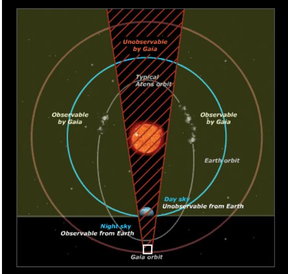
Figure 3. Asteroids blind spot covered by Gaia. Credits: ESA & Medialab
