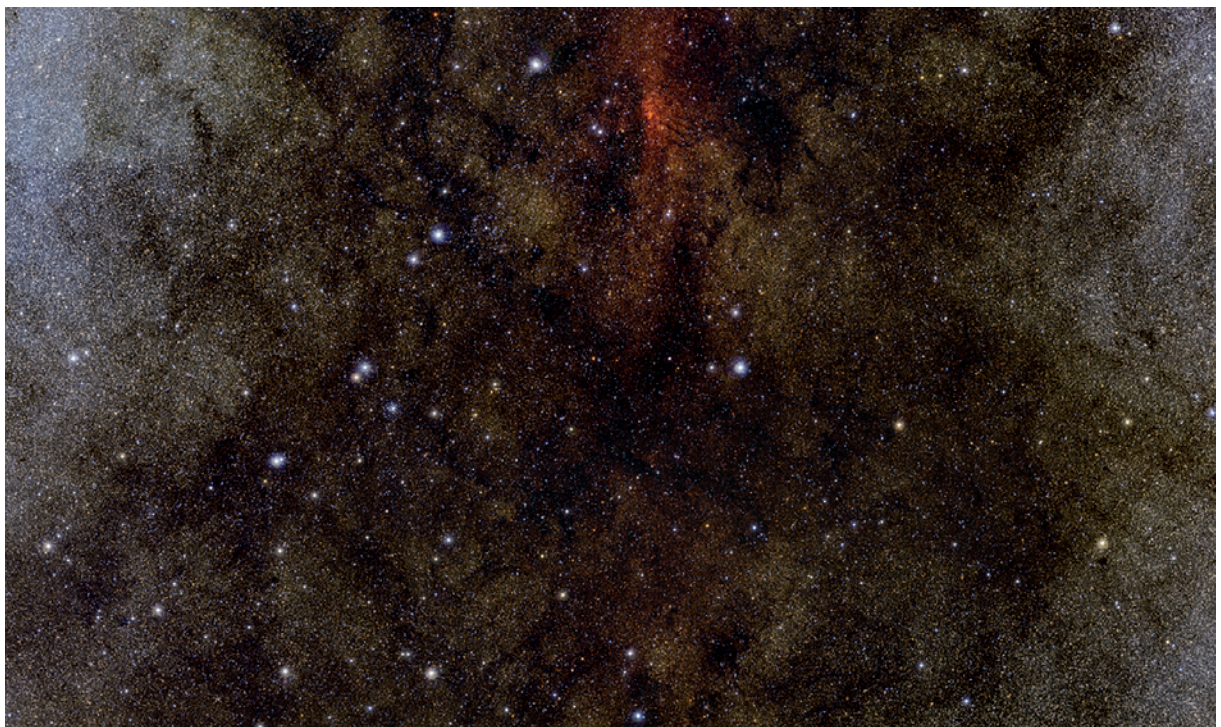
Figure 2. A remarkable ESO VISTA mosaic looking deep into the dusty heart of our own Milky Way galaxy in the constellation of Sagittarius (the Archer). About one million stars are revealed in this picture, most of them not seen in visible light pictures. Credits: ESO/VISTA. Acknowledgment: Cambridge Astronomical Survey Unit
