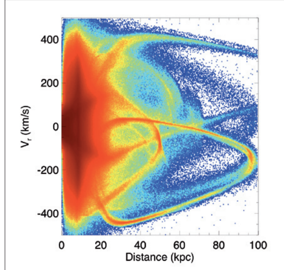
Figure 4. Disrupted dwarf galaxies in the Milky Way halo revealed by Gaia. Streams are revealed easily in the radial velocity-distance plane. Credits: Brown, Velazquez, Aguilar, University of Leiden.
