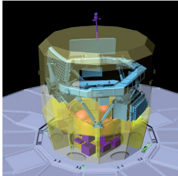
Figure 1. Artist's impression of the Gaia spacecraft. Several components are made transparent to reveal other sections. Credits: ESA/AOES Medialab
