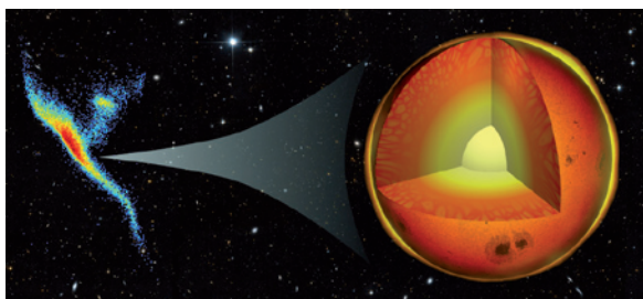
Figure 5. The interior structure of stars from accurate astrometry. Credit: A. Brown, University of Leiden
