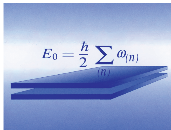
Figure 1. Geometry of two parallel plates in quantum vacuum, initially considered by Hendrik Casimir
